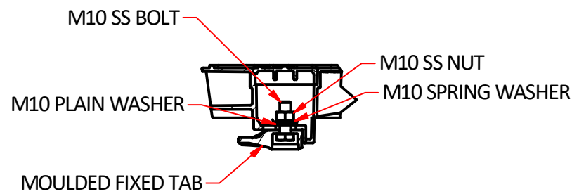
B ( 1:5 ) FIXED LOCK DETAIL
