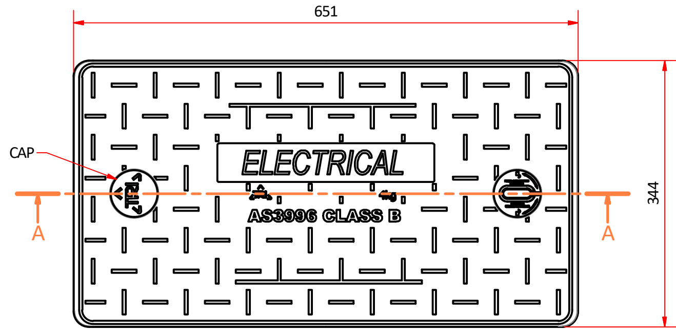
TOP VIEW ( 1:5 )
