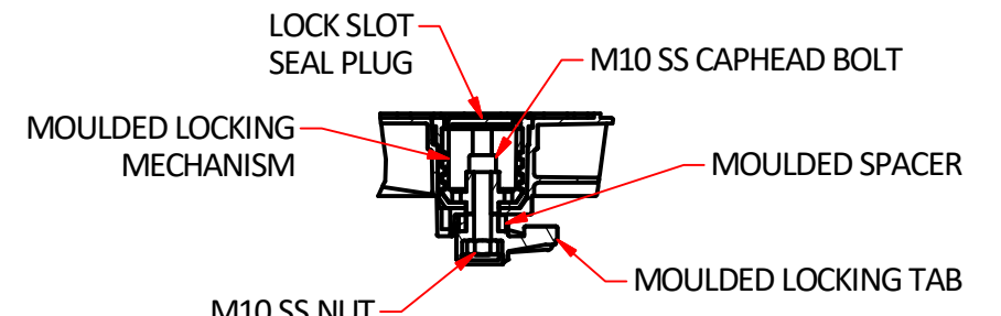
C ( 1:5 ) PIVOTING LOCK DETAIL
