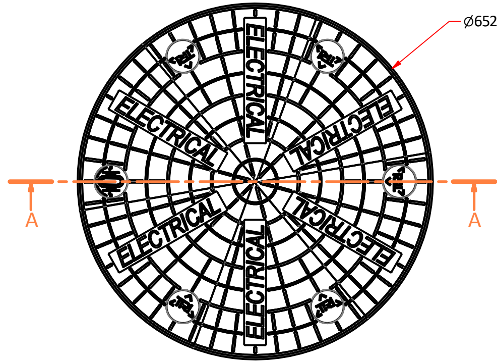
PLAN VIEW ( 1:7 )
