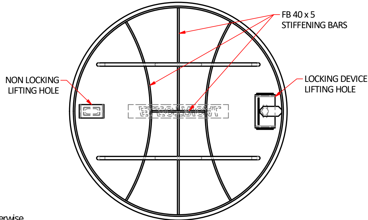
BOTTOM VIEW ( 1:7 )
