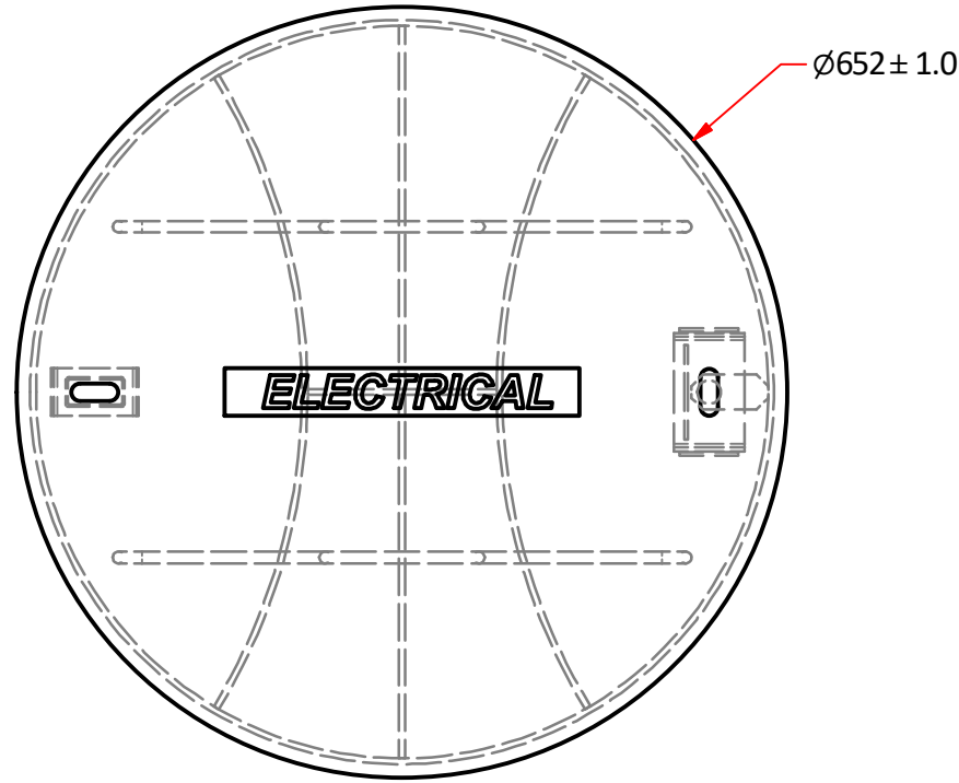
PLAN VIEW ( 1:7 )
