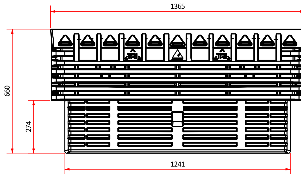
FRONT VIEW ( 1:10 )
