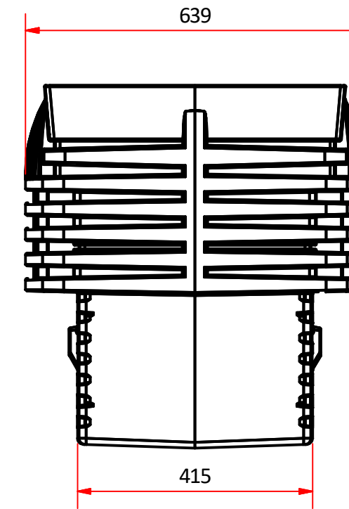
RH END VIEW ( 1:10 )
