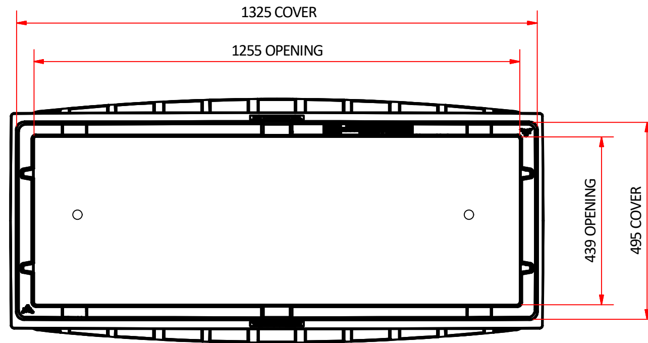
TOP VIEW ( 1:10 )
