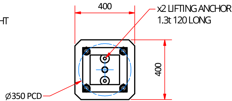
TOP VIEW ( 1:15 )
