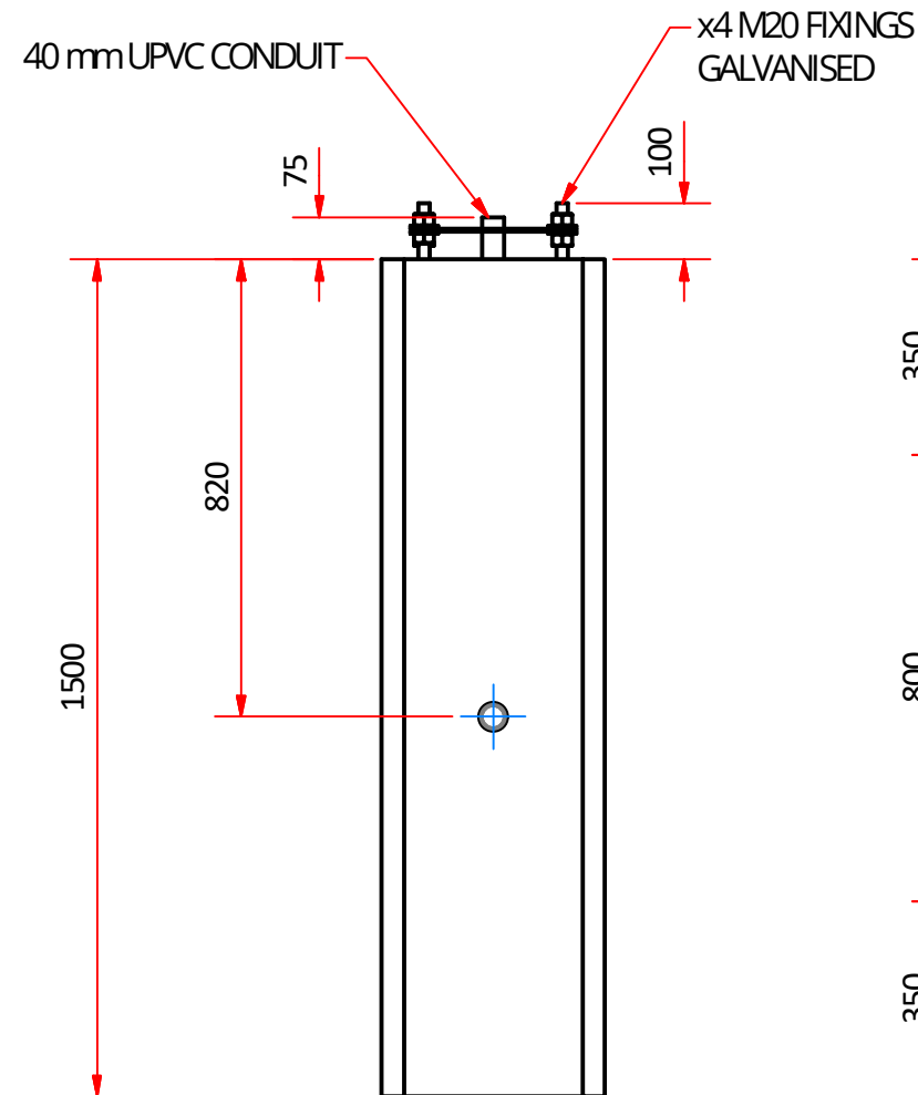
FRONT VIEW ( 1:15 )
